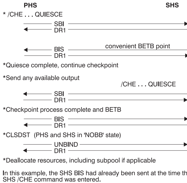
Figure 95. Example 2: Nonsimultaneous Shutdown Using SBI/BIS by Both Half Sessions
