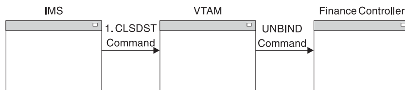
Figure 63. Termination Processing
