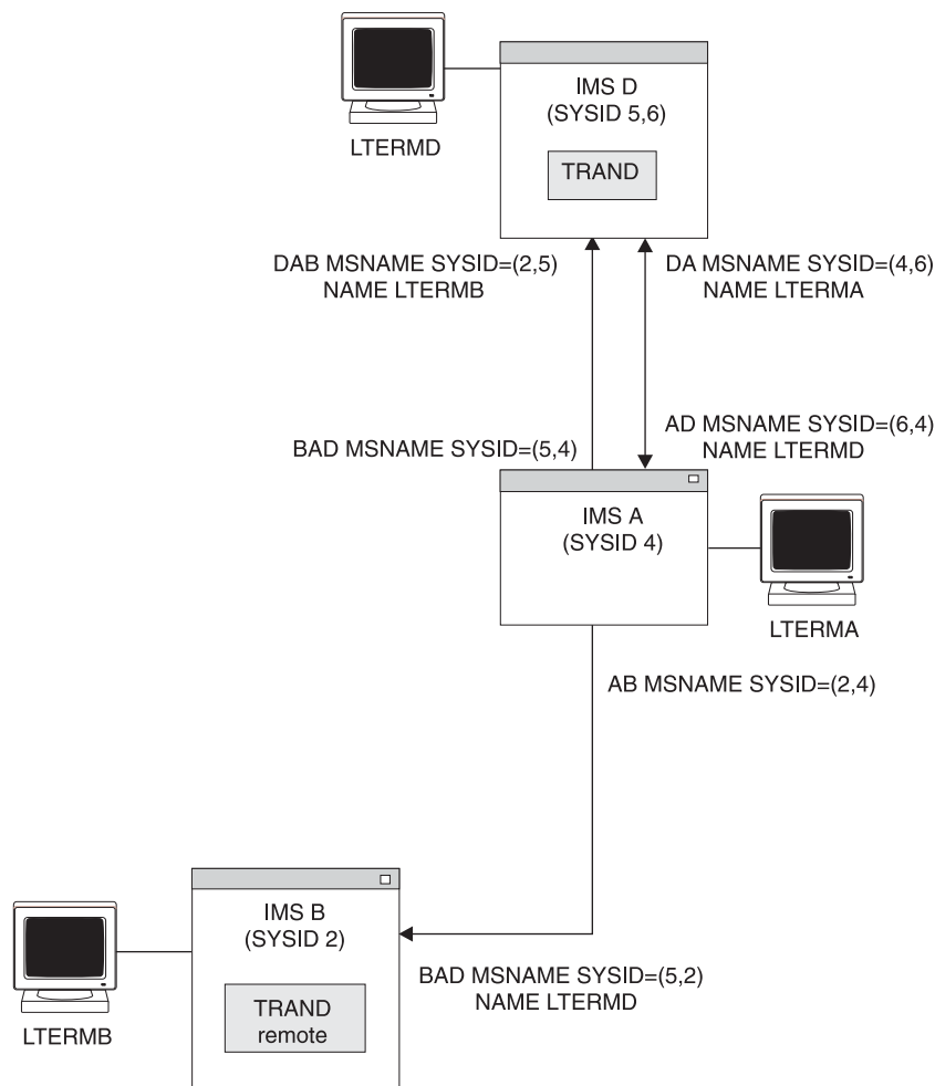
Figure 33. Remote LTERMs
