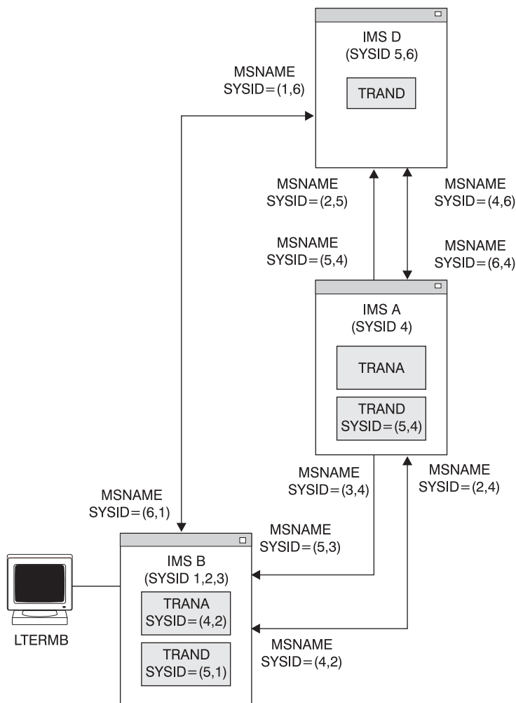
Figure 32. Message Routing
