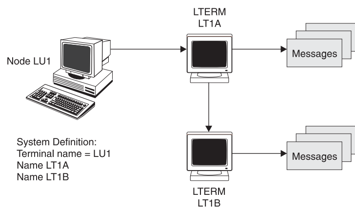
Figure 21. Static Resources
