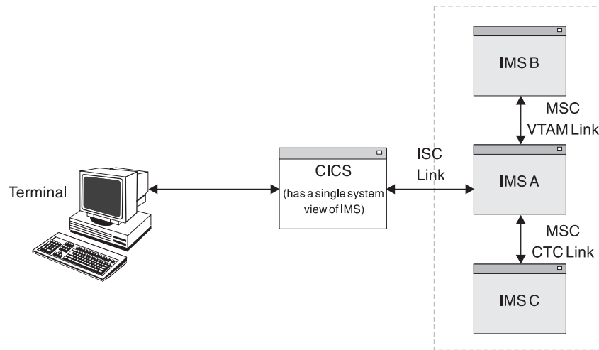
Figure 44. CICS-to-IMS MSC Using ISC
